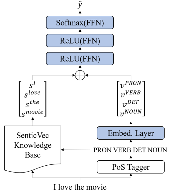
Figure 3: Our SenticVec-based neurosymbolic model. Blue denotes layers with learnable parameters.
