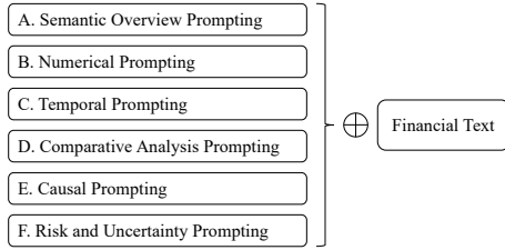
Fig. 1. The proposed financial attribute prompting framework.
